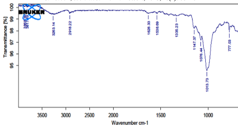
Figure 7.2 FTIR Spectrum of MCP
