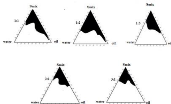
Fig.3. Pseudo-ternary phase diagrams of micro emulsions composed of oil (Oleic acid), surfactant mixture (Smix; propylene glycol: Transcutol P) and water. Shaded area represents the microemulsion region.
