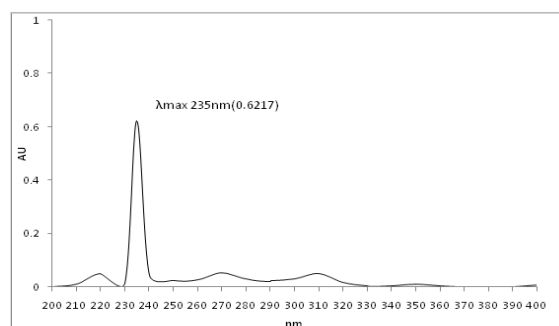
Fig6: Spectrum showing absorption maxima.
