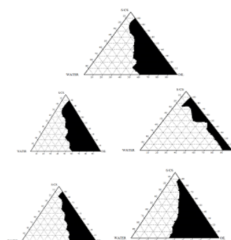
Figure 2: Ternary Phase Diagrams
