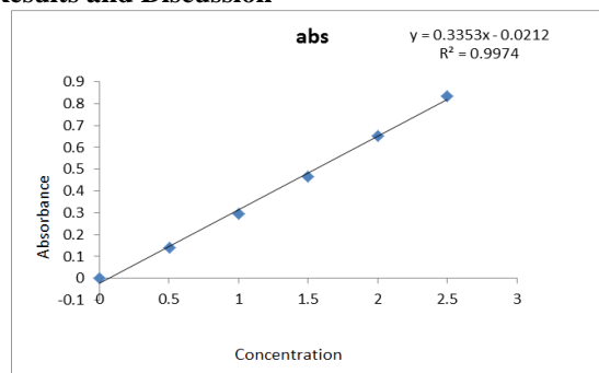
Figure 3: Standard graph of Sotalol in 0.1N HCl
