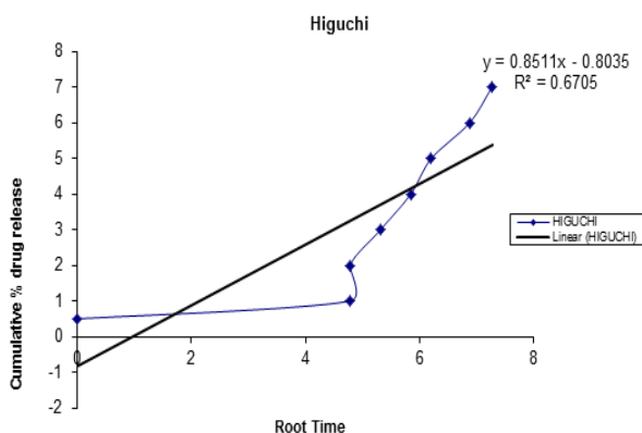
Fig 10: Higuchi release kinetic
