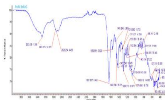
Figure 4: FT-TR Spectrum of Sotalol pure drug
