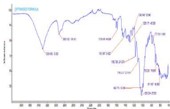
Figure 5: FT-IR Spectrum of Optimized Formulation
