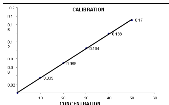
Fig: 2 Calibration curve of lacosamide by first order derivative spectrophotometric method using distilled water
